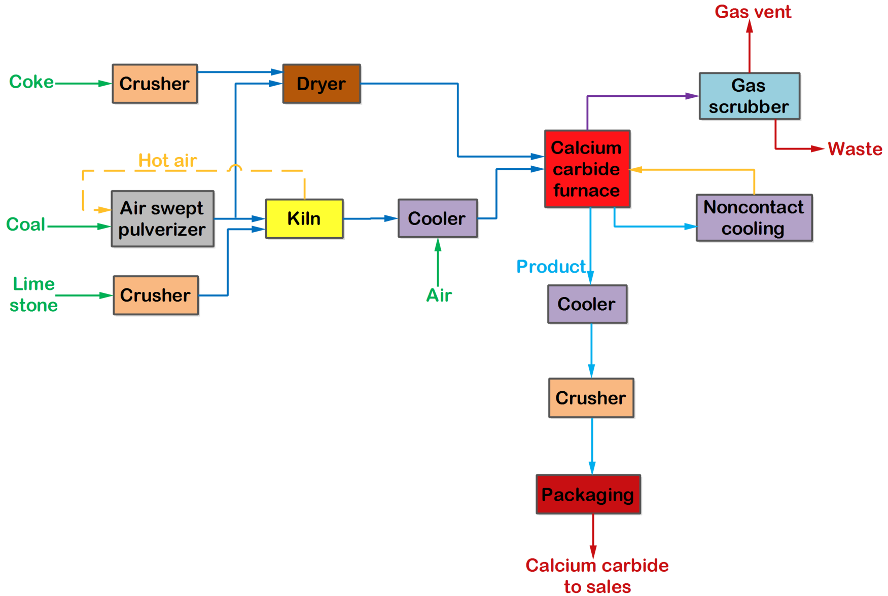
Figure: Manufacture of Calcium carbide by standard process
